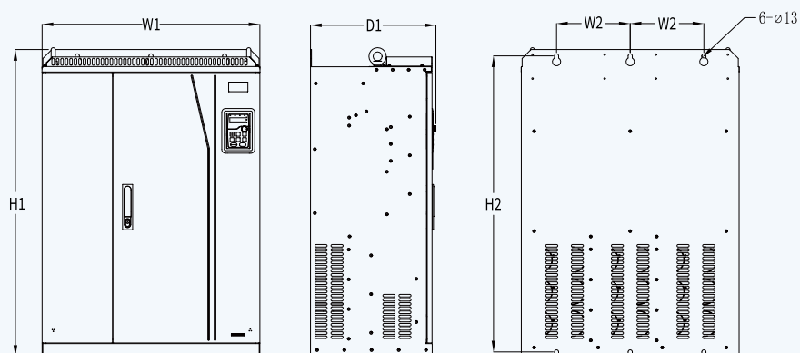
Outline and wall mounting dimensions of 380V 220~315kW VFD models
