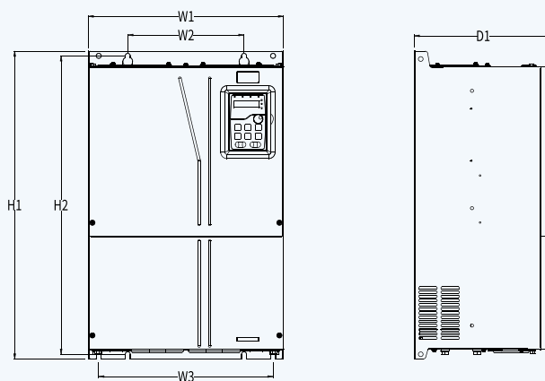
Outline and wall mounting dimensions of 380V 75kW VFD models
