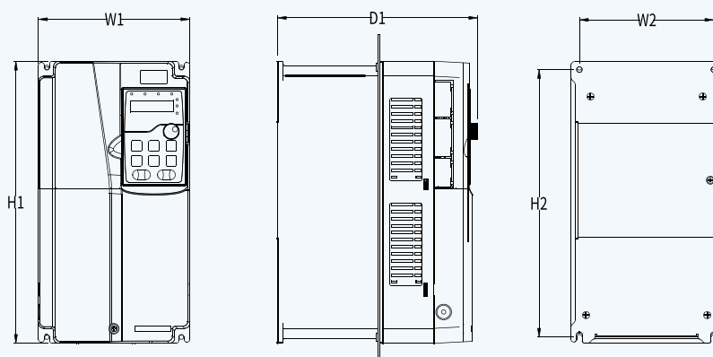
Outline and wall mounting dimensions of 380V 7.5-37kW VFD models
