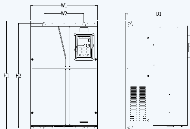
Outline and wall mounting dimensions of 380V 90-110kW VFD models
