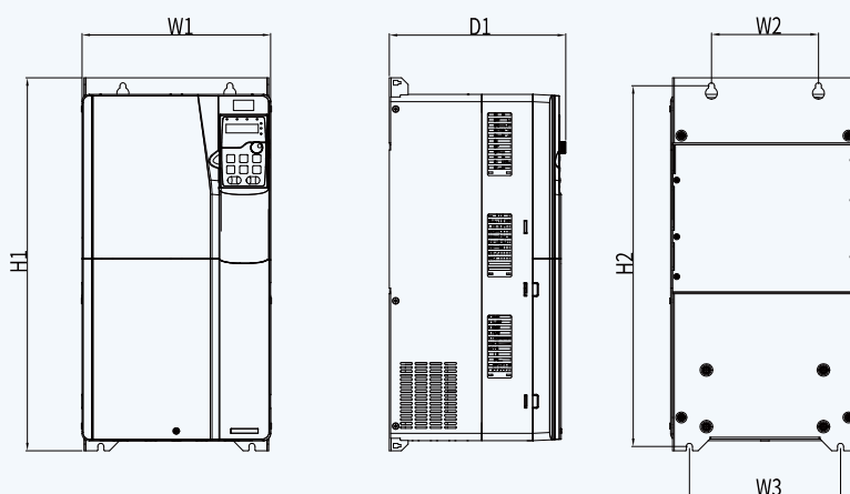
Outline and wall mounting dimensions of 380V 45-55kW VFD models
