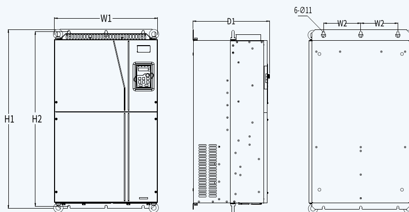
Outline and wall mounting dimensions of 380V 132-200kW VFD models
